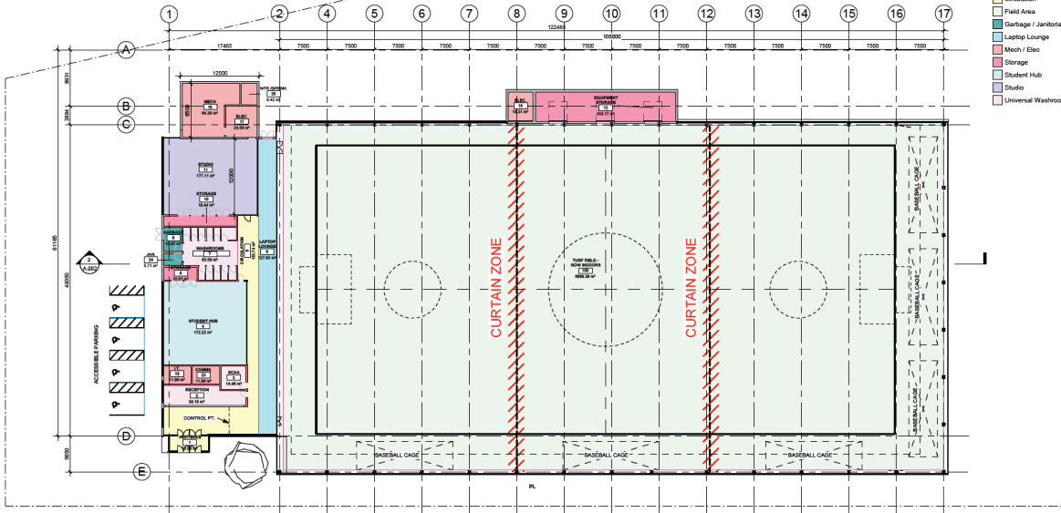
Image 4 – Indicative Ground Plan (source: Workshop + HCMA)
