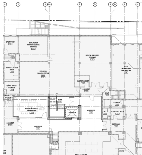
Level 1 Floor Plan - Patient Stair and Elevator, Multi-functional Training Space, Clinic 1 Entrance
