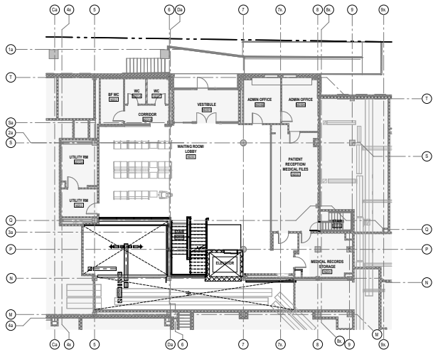
Patient Entrance and Waiting at Mezzanine Level - New Patient Stair and Elevator
