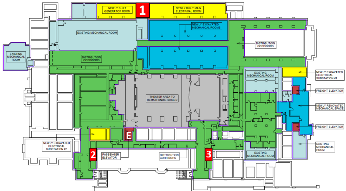
Elevator locations at Hart House – Existing and Proposed
