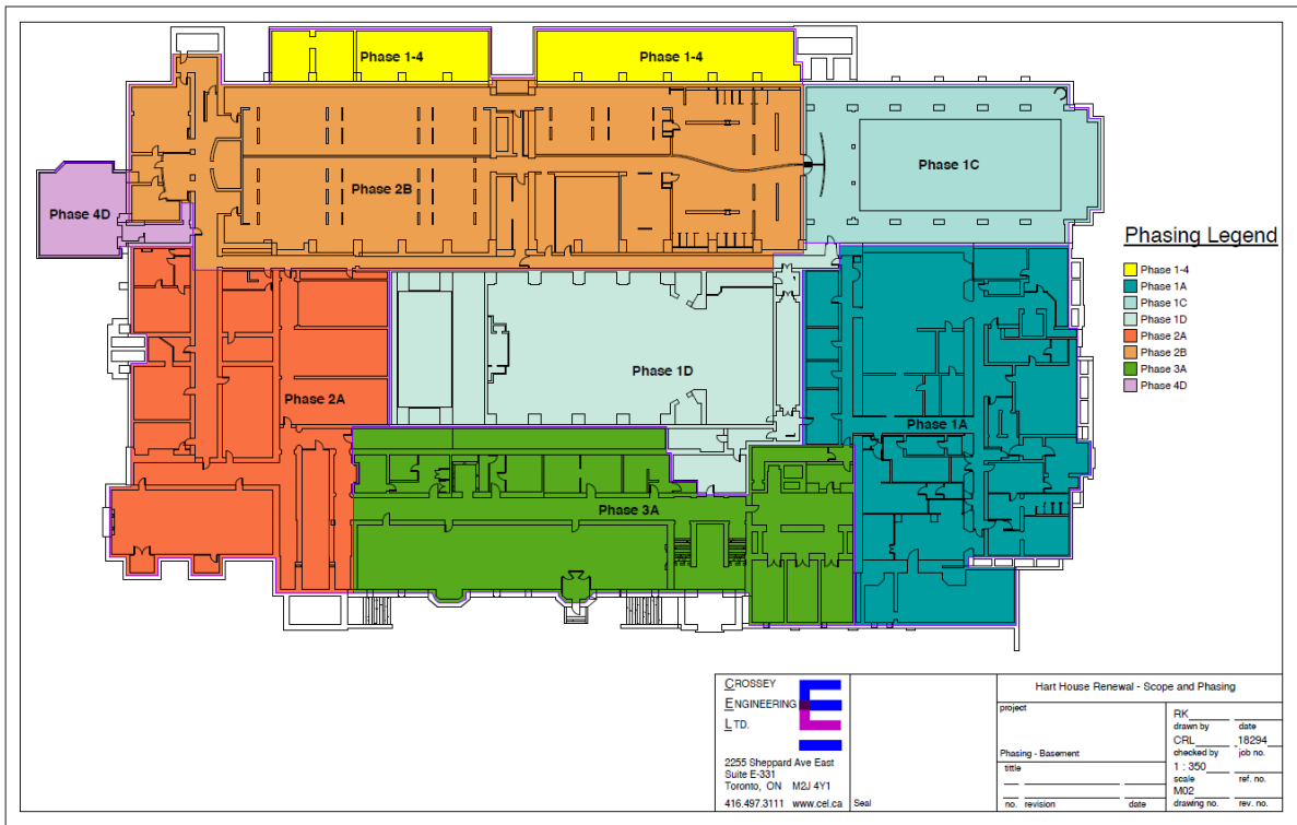
Scope and Phasing –Basement local phases
