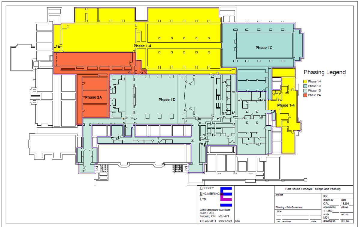
Scope and Phasing –Sub-basement local phases
