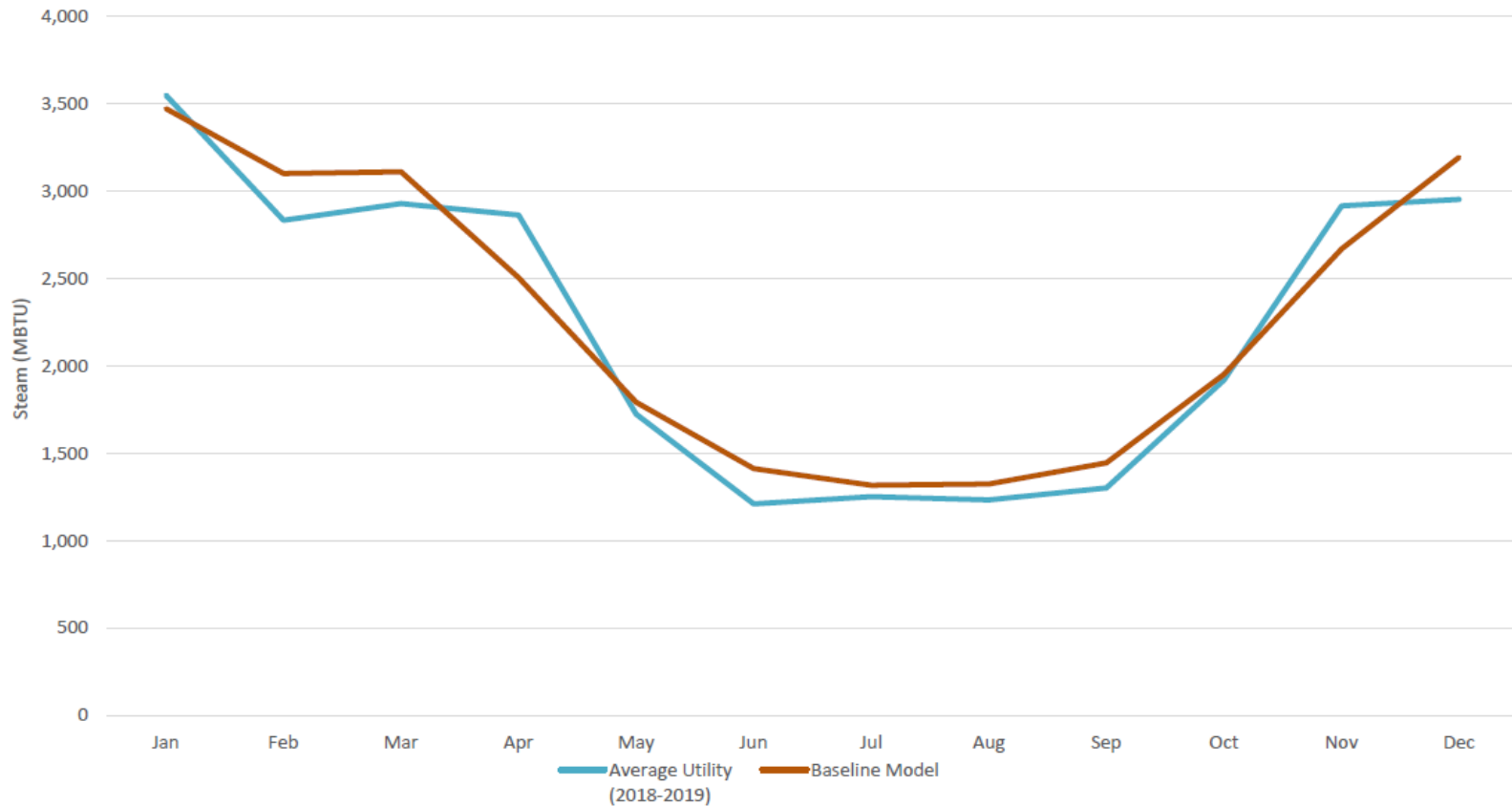
Modelled vs Historical Steam Consumption
