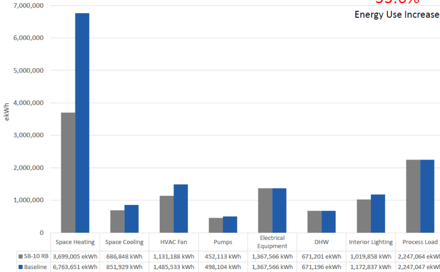
SB-10 Reference Building vs Baseline Building
