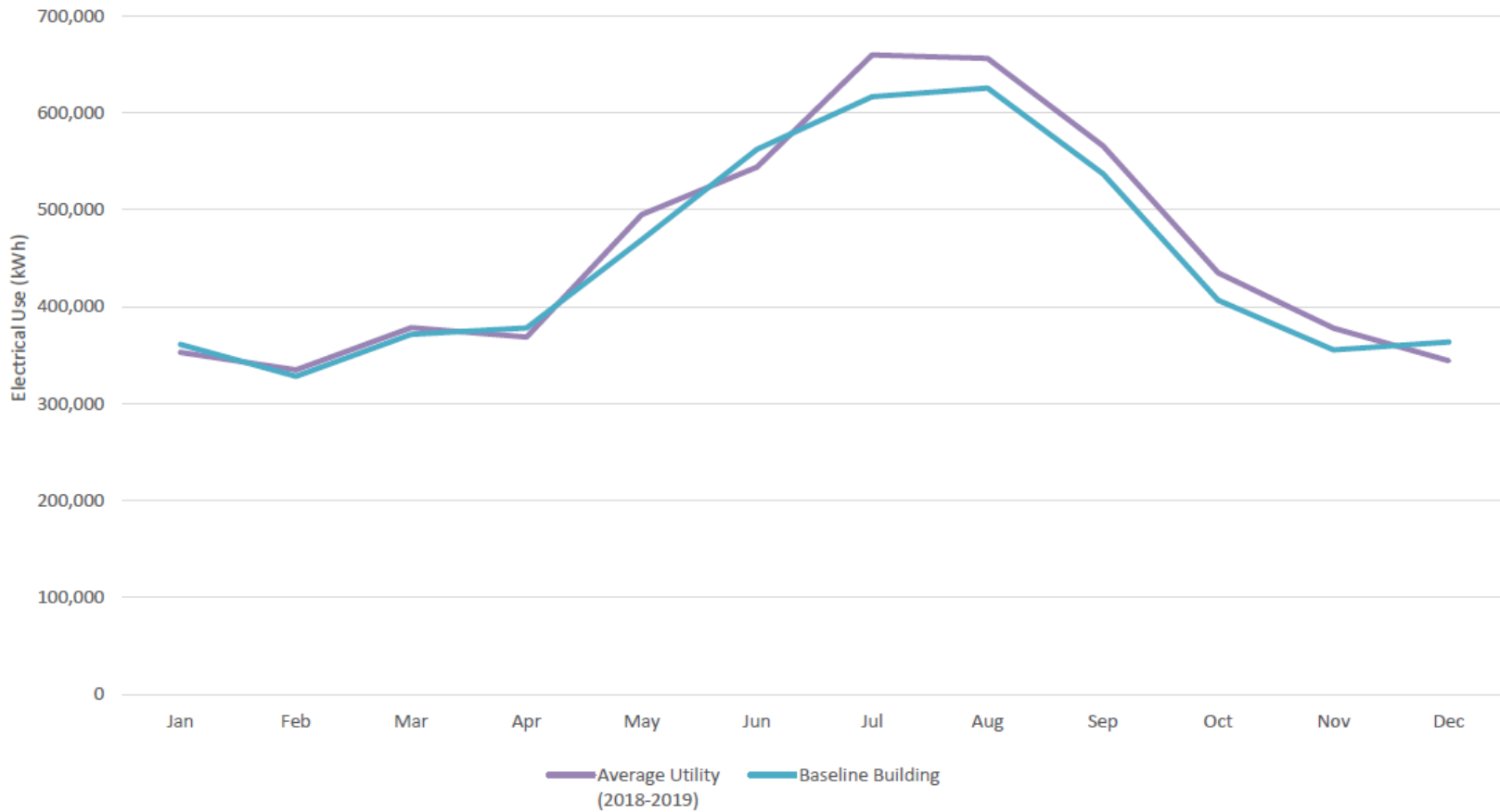
Modelled vs Historical Electricity Consumption
