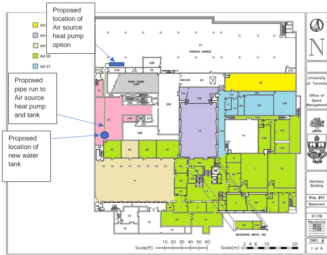
Figure 22 Proposed location of the DHW Heat Pump system
