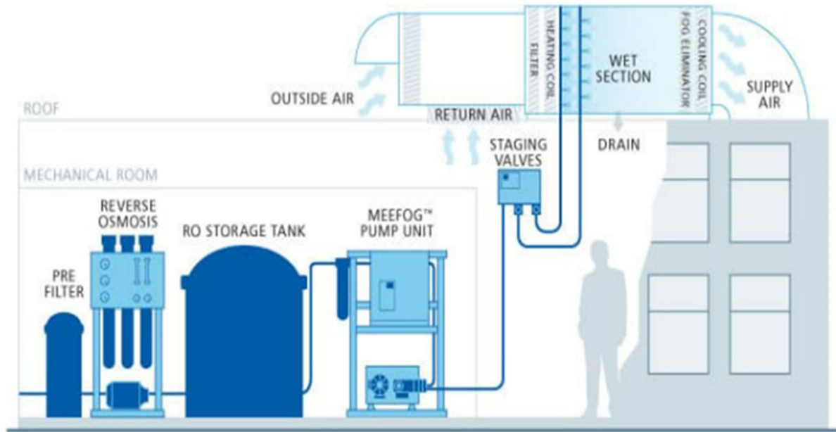
Figure 28: Typical Adiabatic Schematic
