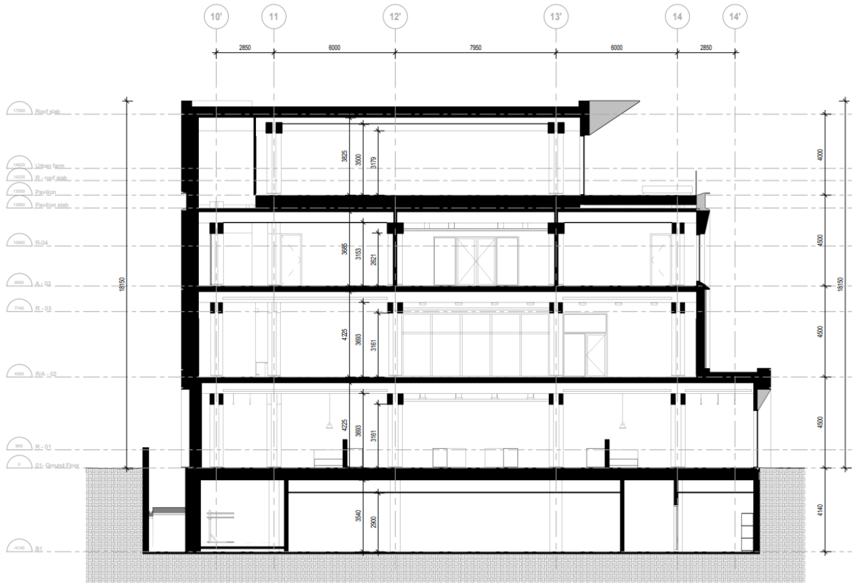
Figure 12: Profile section, centre Pavillion structure
