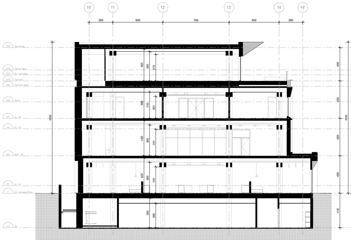
Figure 12: Profile section, centre Pavilion structure
